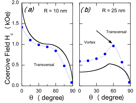
Fig. 3. Angular dependence of the coercivity, H_c , in a Ni nanotube with L = 0.5 \mu\text{m} , \beta = 14/30 , and (a) R = 10 \text{ nm} , and (b) R = 25 \text{ nm} .
