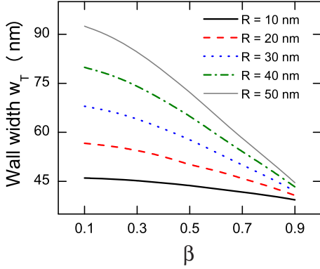
Fig. 2. Domain wall width as a function of \beta for the T mode of magnetization reversal.
