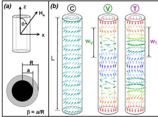
Fig. 1. (a) Geometrical parameters of a nanotube. (b) Magnetization reversal modes in nanotubes. The arrows represent the orientation of magnetic moments within the tube. Left: coherent-mode rotation, C. Center: vortex-mode rotation, V, with a domain wall of thickness w_V . Right: transverse-mode rotation, T, with a domain wall of thickness w_T .
