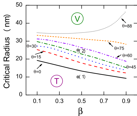
Fig. 4. Critical radius as a function of \beta for different angles. Points 1 and 2 are discussed in the text.
